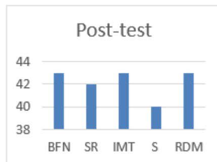
Gambar 1. Hasil Postt-test
