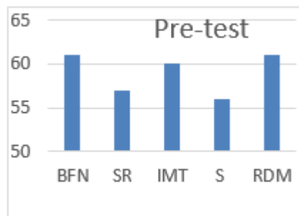
Gambar 1. Hasil Pre-test
