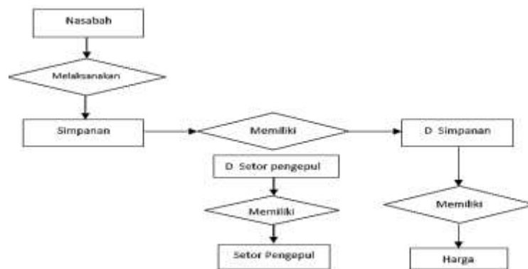
Gambar 3. Tampilan Flowchart
