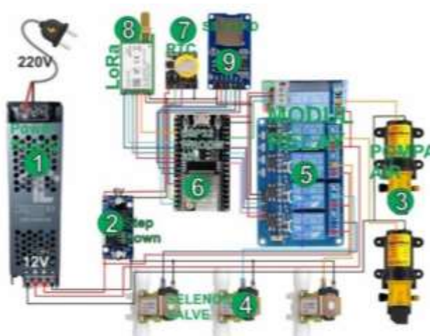
Gambar 2.3 Wiring Diagram
