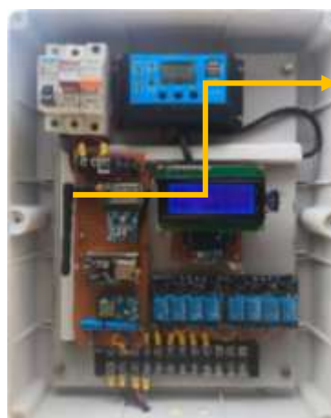
Gambar 4.4 LoRa E32-433T20D
